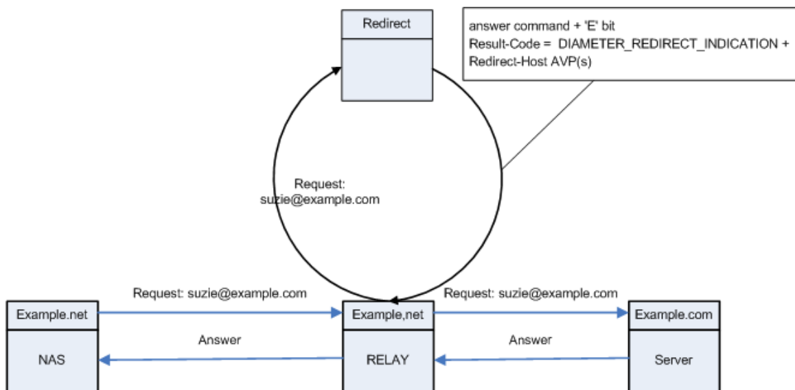
Fig. 3 Diameter Redirect agent Example (Source: Mobiecents project)
