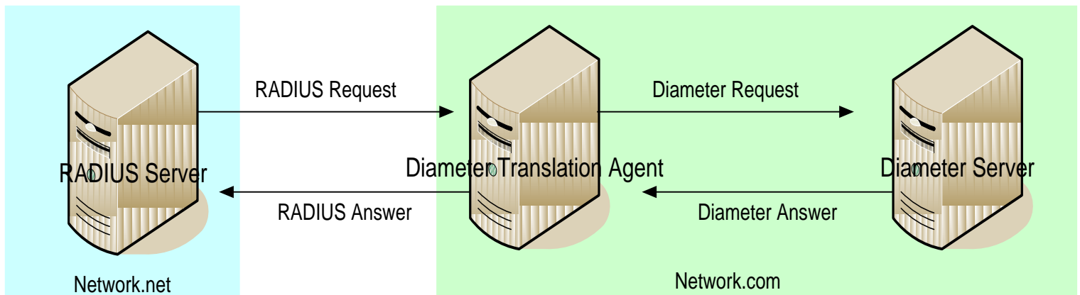
Fig. 4 Diameter Translation agent Example
