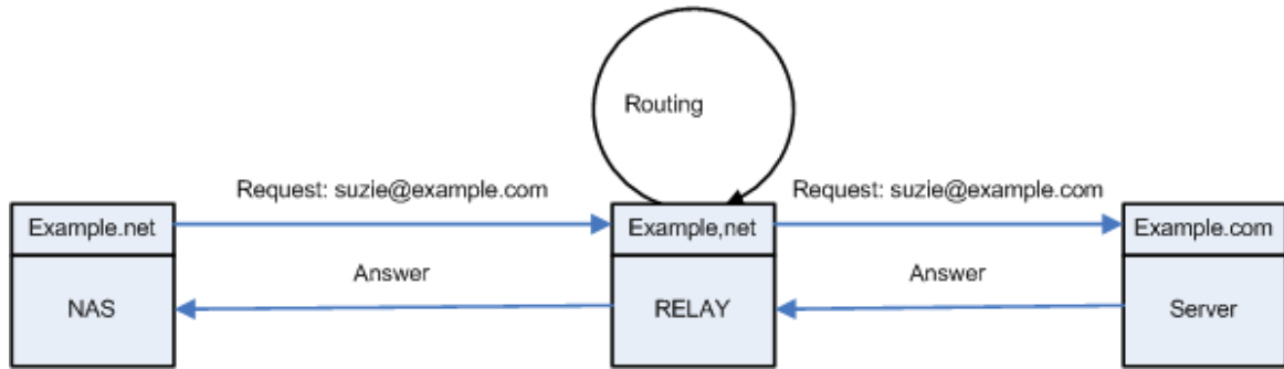
Fig. 1 Diameter Relay agent Example (Source: Mobiecents project)
